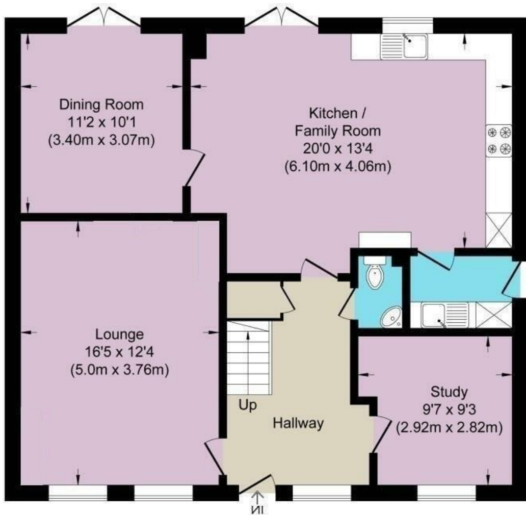
Ground Floor
