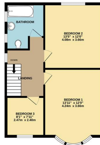
1ST FLOOR 551 sq.ft. (51.2 sq.m.) approx.
