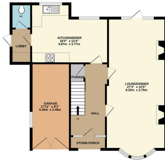
GROUND FLOOR 835 sq.ft. (77.6 sq.m.) approx.
