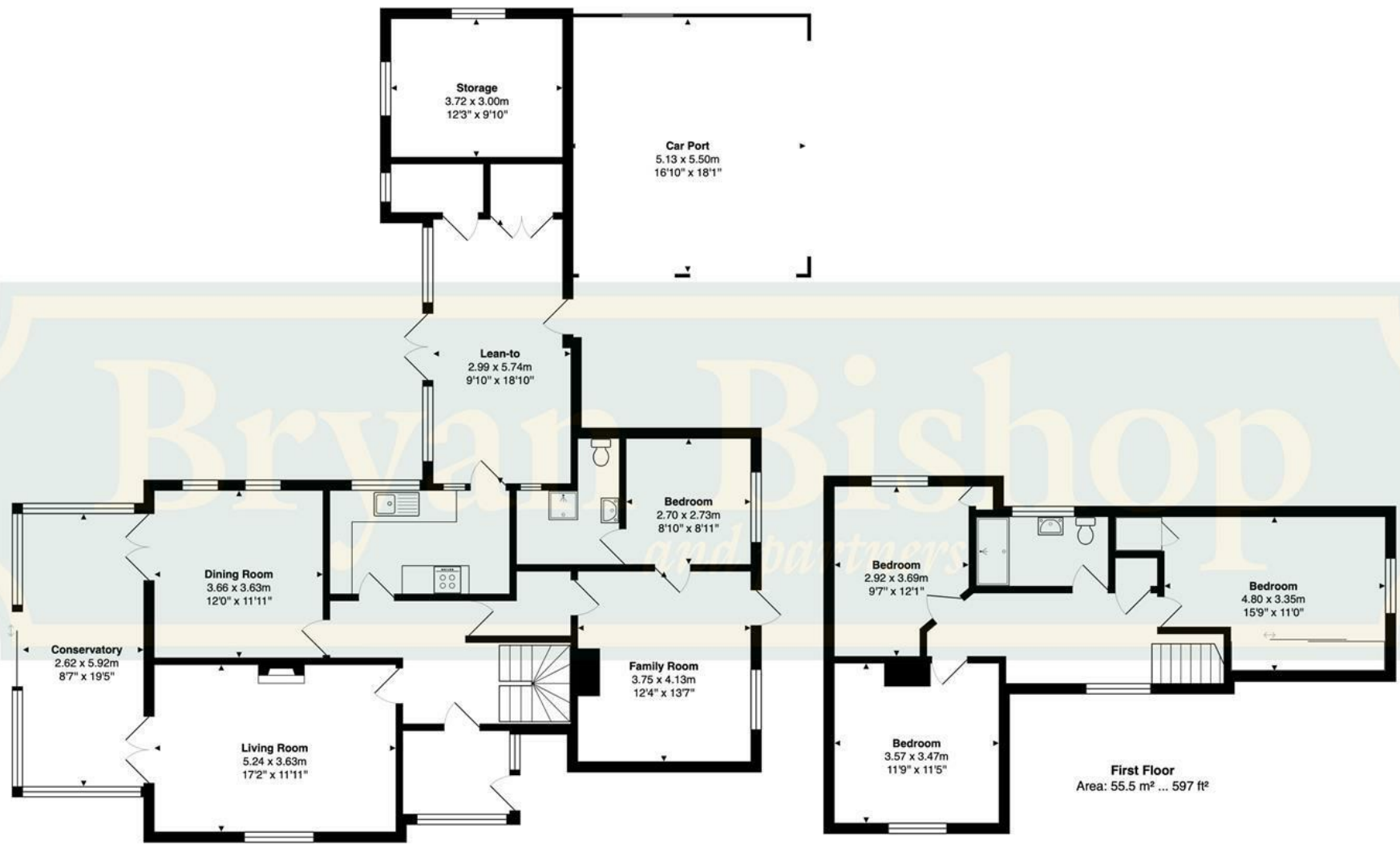
Ground Floor Area: 140.5 m 2 ... 1513 ft 2
