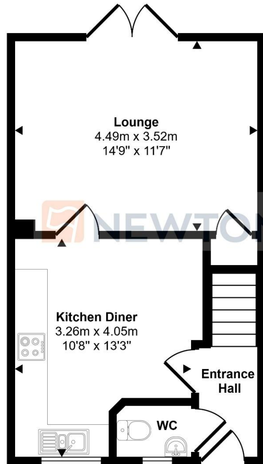
Ground Floor Approx 35 sq m / 375 sq ft
