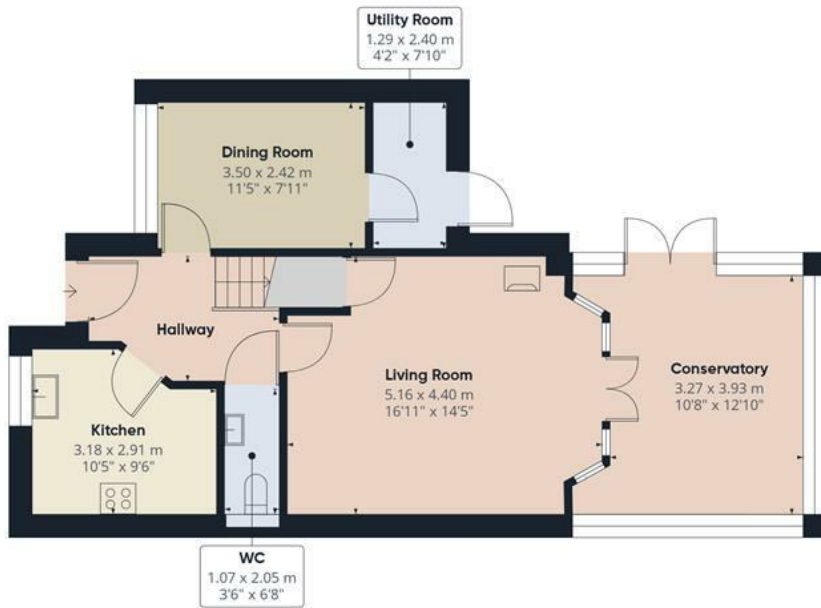
Floor 0
