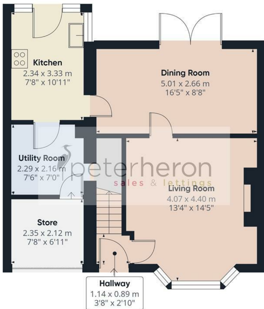
Ground Floor
