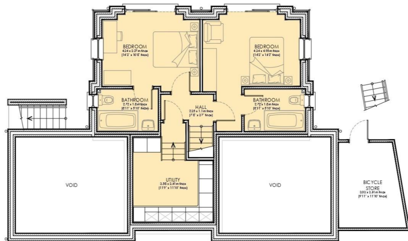
LOWER GROUND FLOOR 1:100 GIA: 53.96m 2
