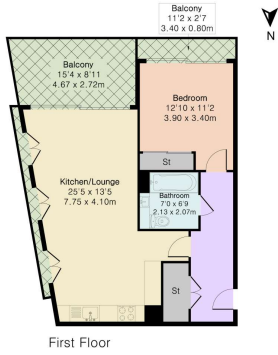
Floor Plan
