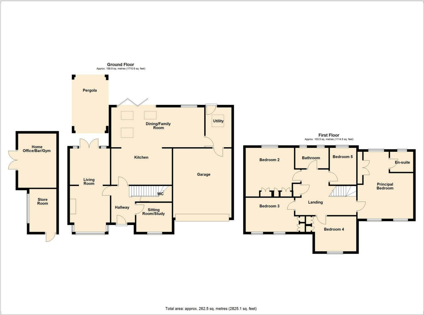
Floor Plan
