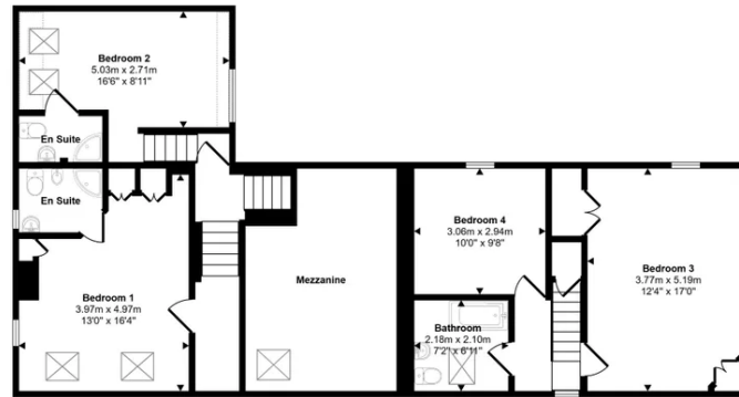
First Floor Approx 87 sq m / 941 sq ft
