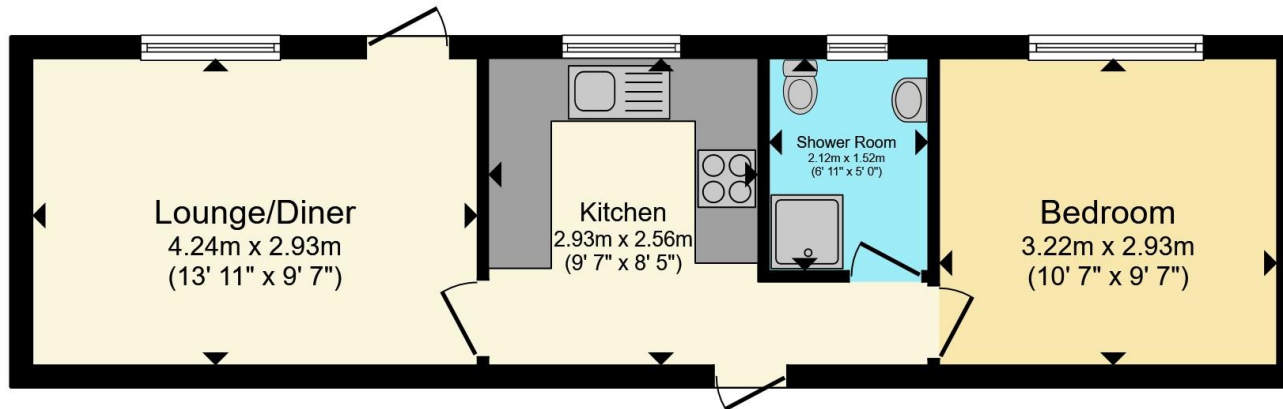
Floor Plan
