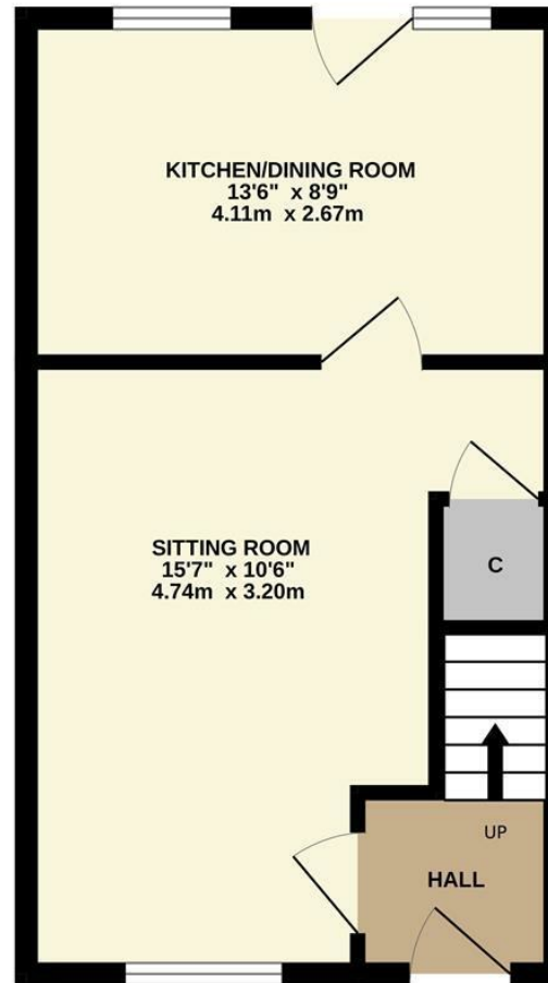
GROUND FLOOR 328 sq.ft. (30.5 sq.m.) approx.
