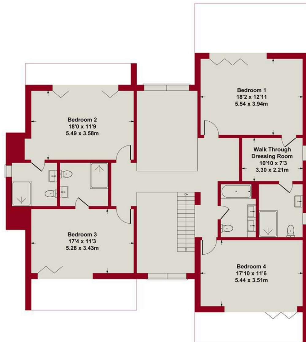
FIRST FLOOR
