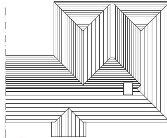
ROOF PLAN 1:100
