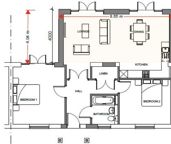
GROUND FLOOR PLAN 1:100
