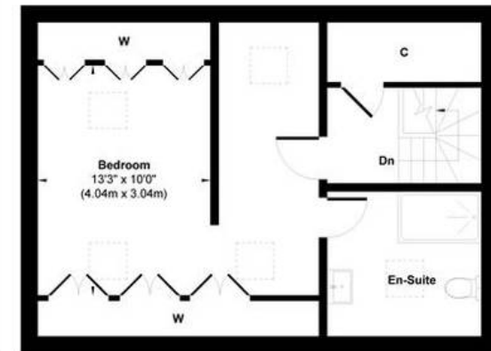
Second Floor Approximate Floor Area 465 sq.ft (43.18 sq.m)
