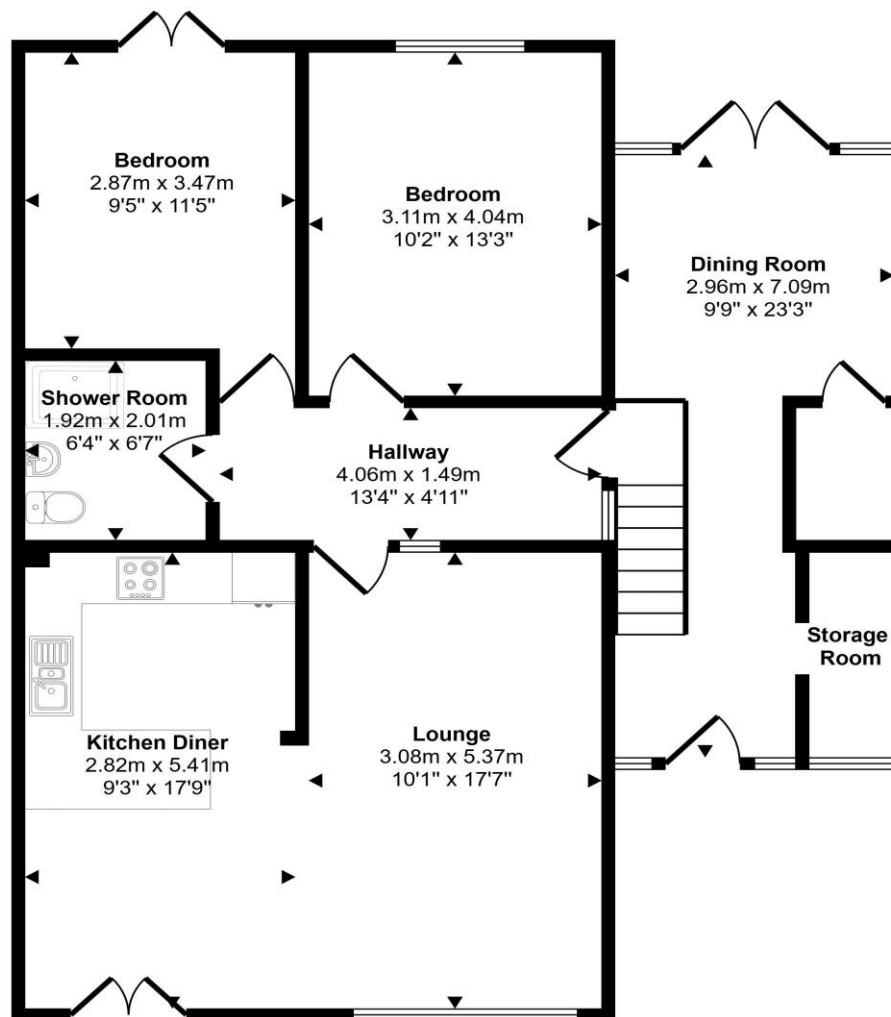
Floorplan
