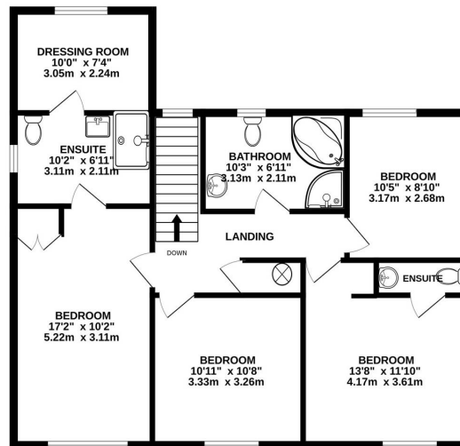
1ST FLOOR 852 sq.ft. (79.1 sq.m.) approx.
