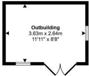
Outbuilding Approx 10 sq m / 103 sq ft
