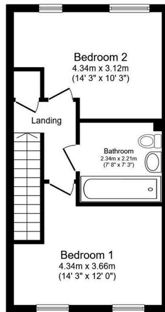
First Floor Floor area 37.2 sq.m. (400 sq.ft.)
