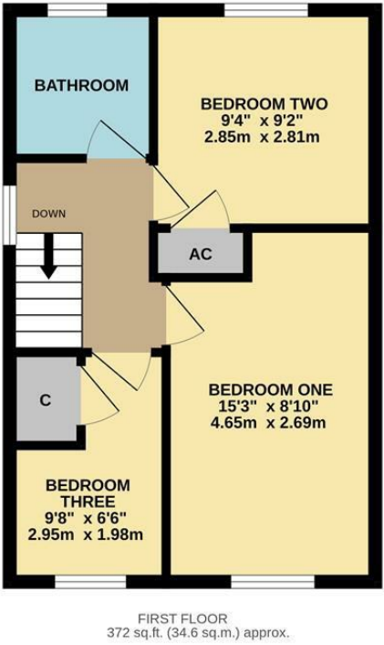
TOTAL FLOOR AREA : 1010 sq.ft. (93.8 sq.m.) approx. Whilst every attempt has been made to ensure the accuracy of the floorplan contained here, measurements of doors, windows, rooms and any other items are approximate and no responsibility is taken for any error, omission or mis-statement. This plan is for illustrative purposes only and should be used as such by any prospective purchaser. The services, systems and appliances shown have not been tested and no guarantee as to their operability or efficiency can be given. Made with Metropix ©2025
