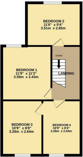
1ST FLOOR
