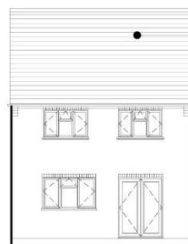
South Elevation
