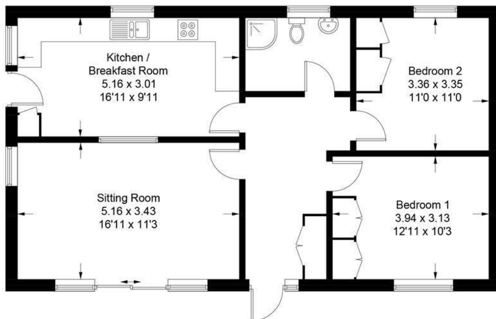
Outbuilding - First Floor
