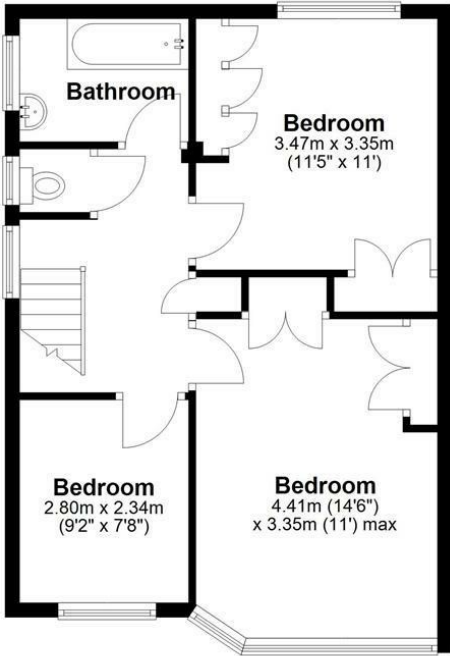
First Floor Approx. 48.2 sq. metres (518.5 sq. feet)
