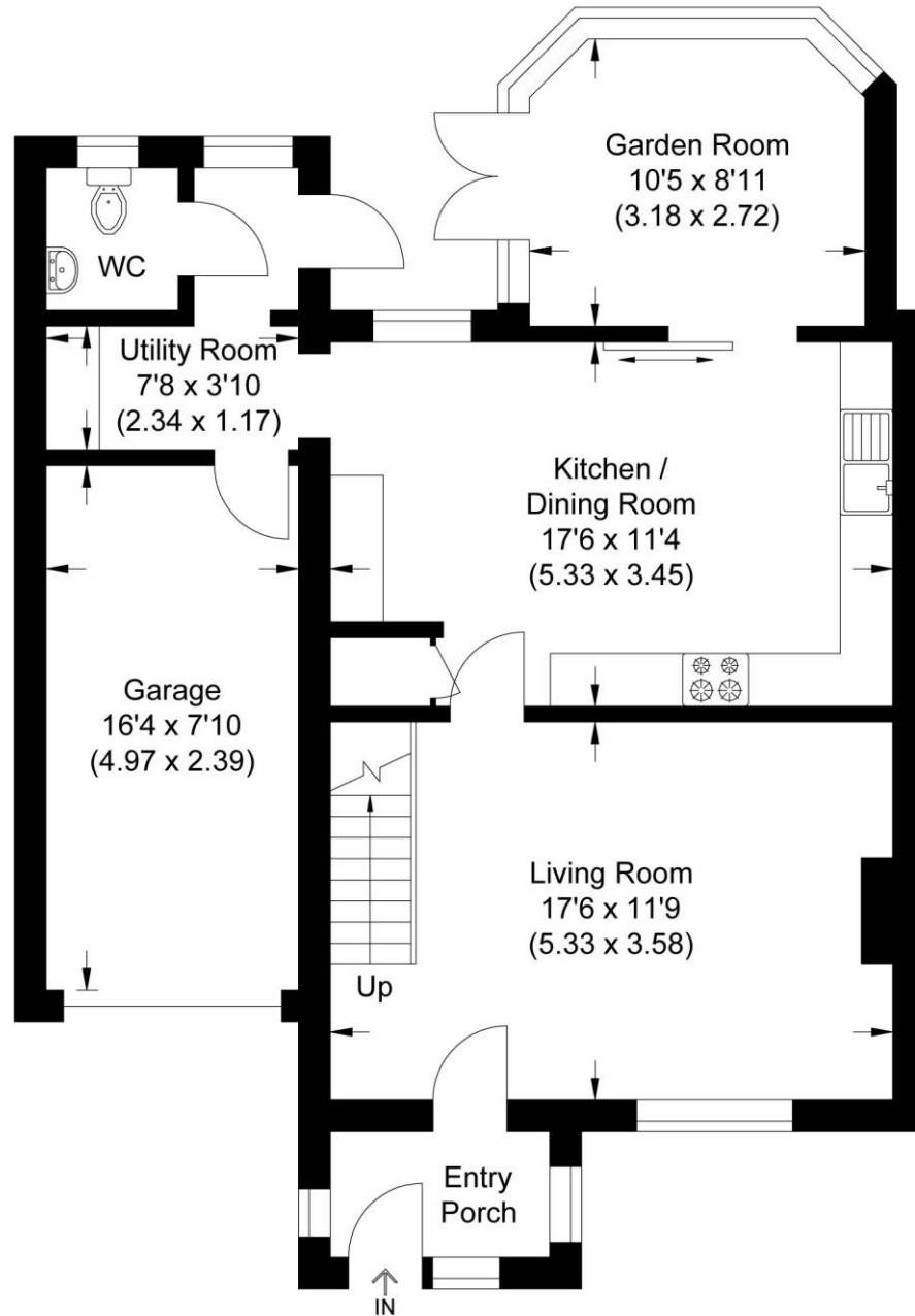
Ground Floor
