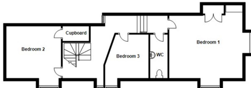
Second Floor
