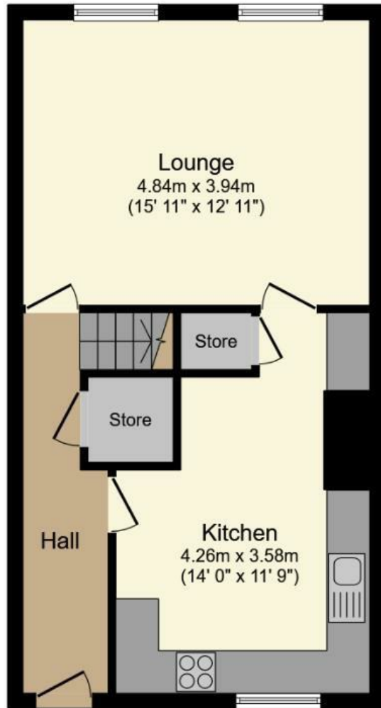
Ground Floor Floor area 45.8 sq.m. (493 sq.ft.)
