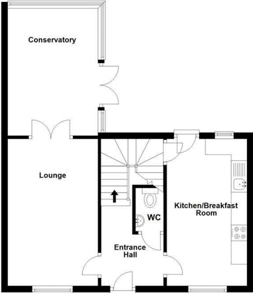
Ground Floor Approx. 47.1 sq. metres (506.8 sq. feet)
