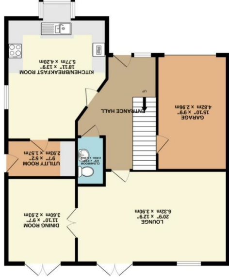
GROUND FLOOR 946 sq.ft. (87.9 sq.m.) approx.
