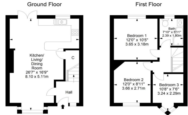
Approximate gross internal floor area 77.5 sq m/ 834.2 sq ft Whilst every care has been taken to ensure accuracy, dimensions are approximate and for illustrative purposes only. All rights reserved.
