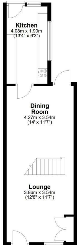
Ground Floor
