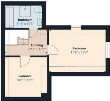
Floor 2 Building 1
