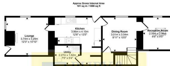
Ground Floor Approx 54 sq m / 581 sq ft
