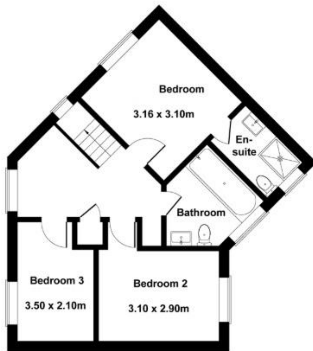
FIRST FLOOR
