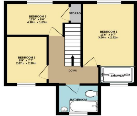
1ST FLOOR 384 sq.ft. (35.7 sq.m.) approx.
