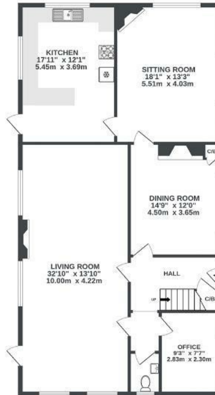
GROUND FLOOR 1264 sq.ft. (117.5 sq.m.) approx.
