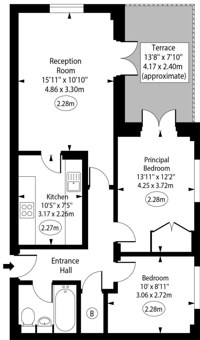
Third Floor
