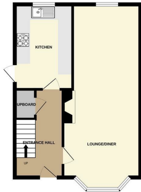
GROUND FLOOR
