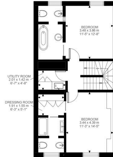
Second Floor 634 ft 2
