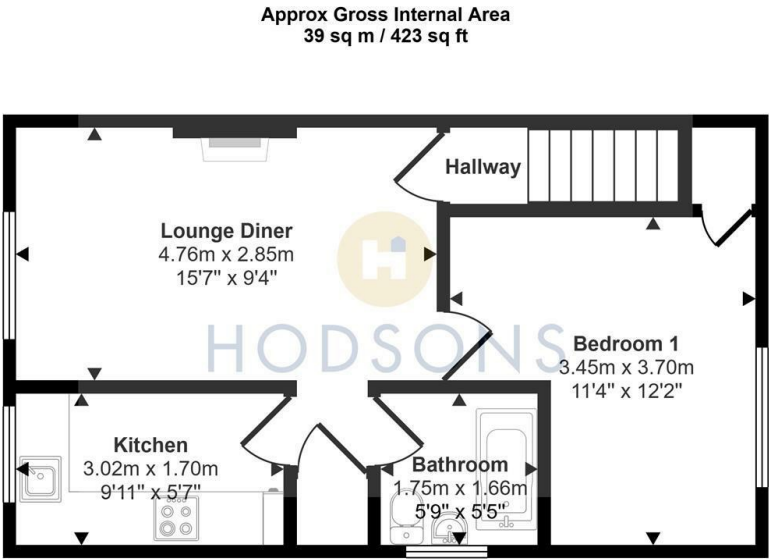
Floorplan
