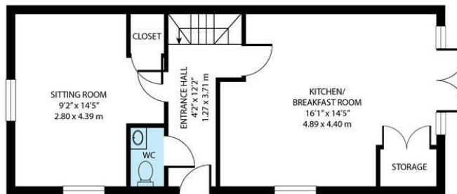
GROUND FLOOR
