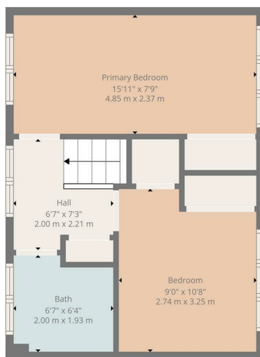
1st Floor
