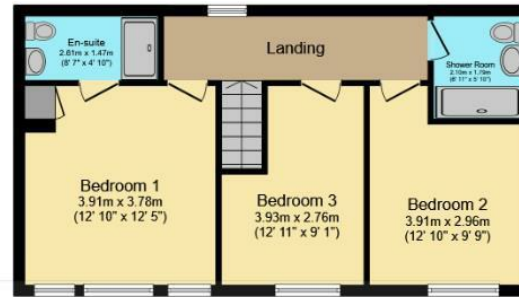
First Floor Floor area 51.5 sq.m. (554 sq.ft.)
