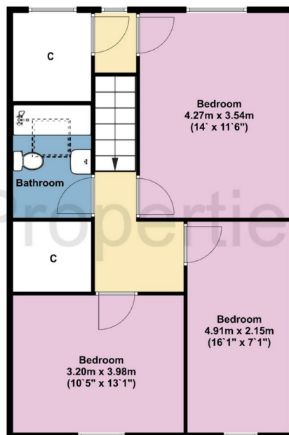
First Floor Approx 68.00 Sq meters (732.00 Sq feet).
