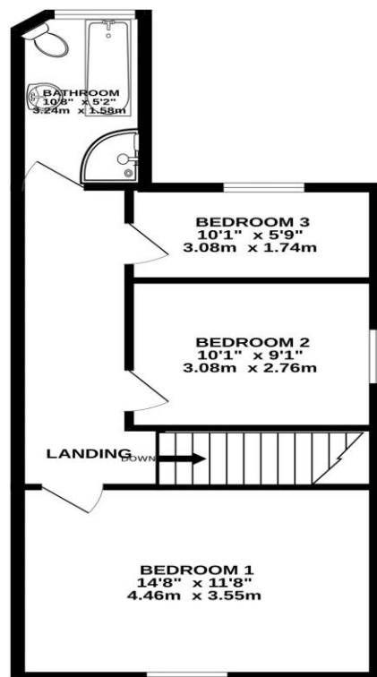
1ST FLOOR 494 sq.ft. (45.9 sq.m.) approx.
