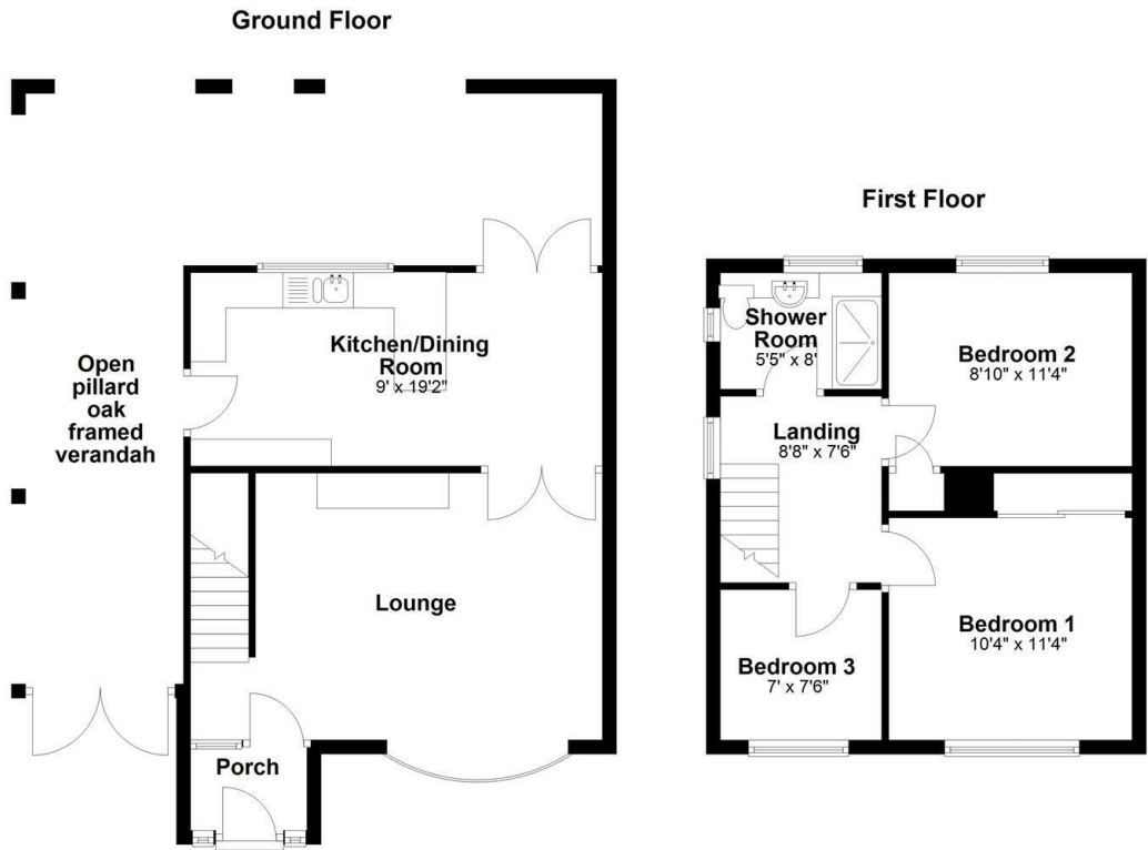
Total area: approx. 1231.8 sq. feet
