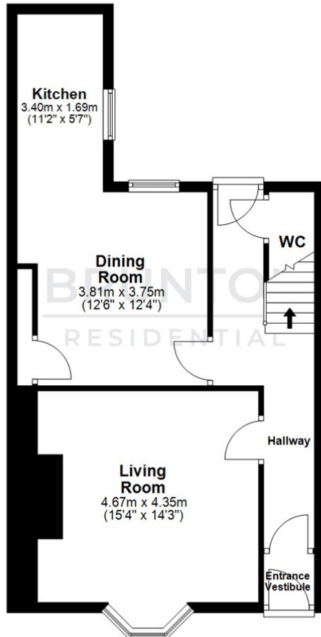
Ground Floor Approx. 53.4 sq. metres (574.3 sq. feet)
