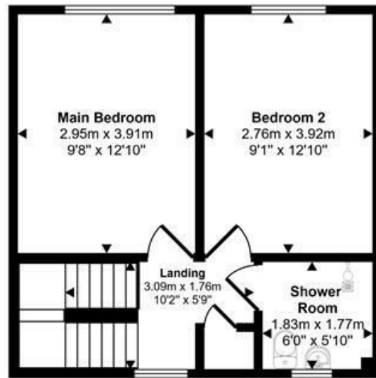
First Floor Approx 34 sq m / 367 sq ft
