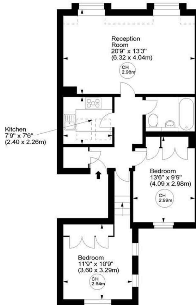
Fourth Floor
