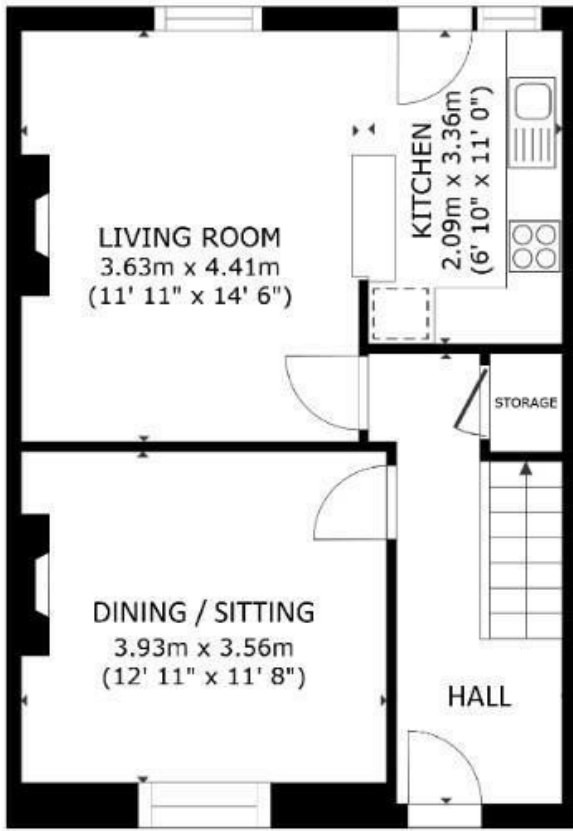
FLOOR 1
